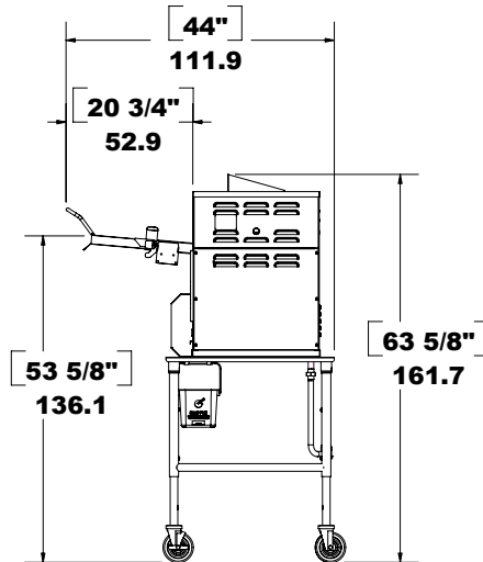
HIGH POSITION
