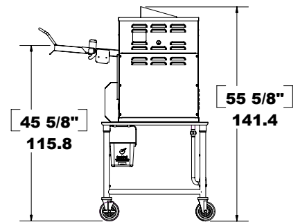
LOW POSITION
